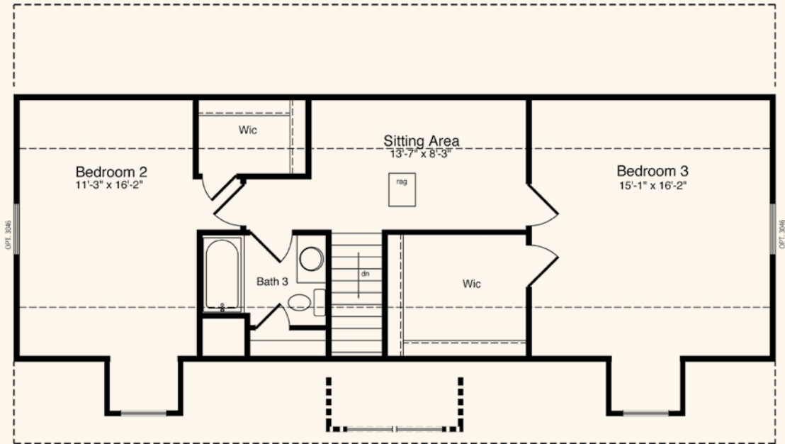
OPT. 8'-0" DORMER suggested second floor
